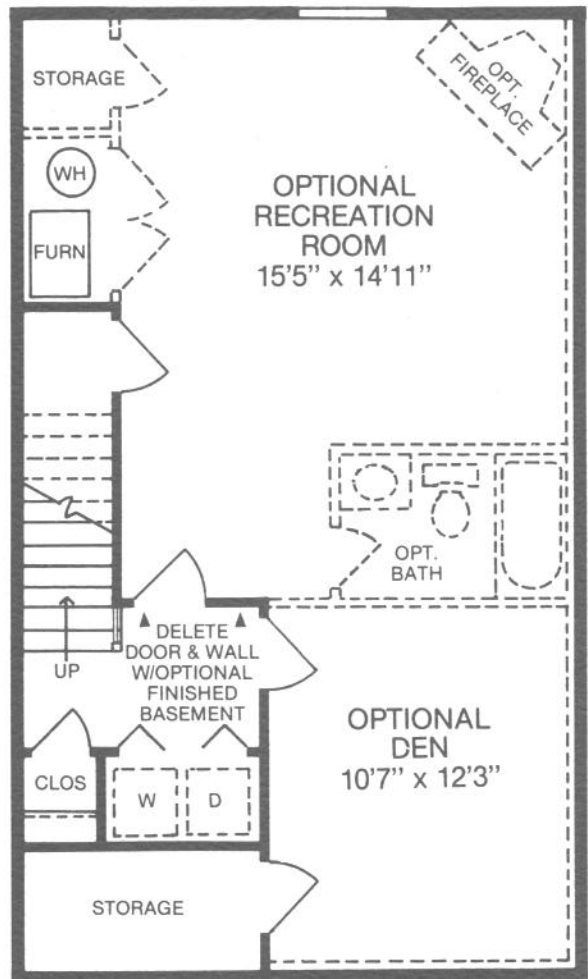
ENGLISH BASEMENT
