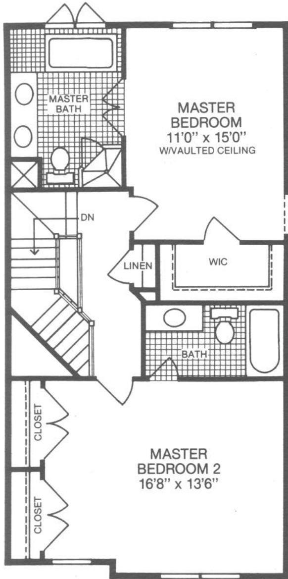
SECOND FLOOR ELEVATION 2 W/2 BEDROOMS
