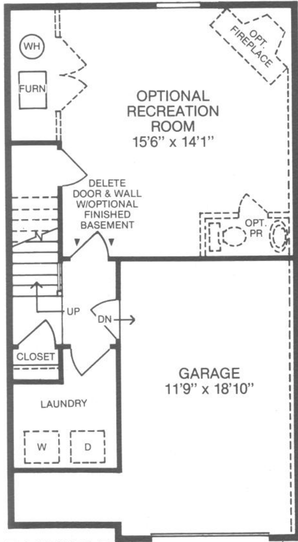
BASEMENT W/GARAGE
