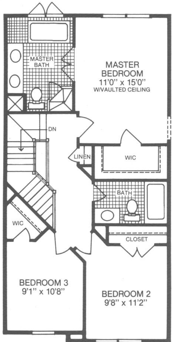
SECOND FLOOR ELEVATION 2 W/3 BEDROOMS
